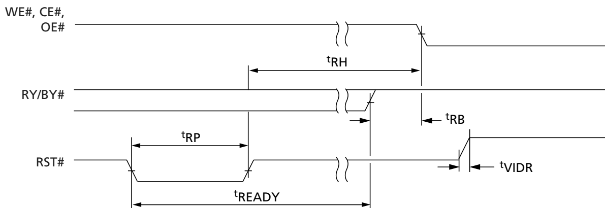
Figure 16: Reset/Block Temporary Unprotect AC Waveforms
